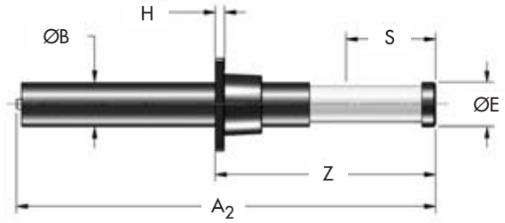
FF (FLANGE FRONT)
